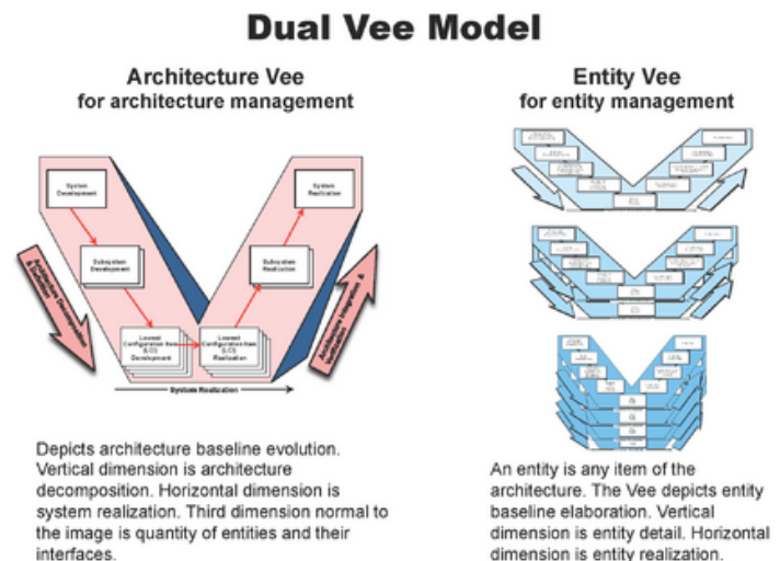
Figure 2a. The Dual Vee Model (2a) (Forsberg, Mooz, Cotterman 2005). Reprinted with permission of John Wiley & Sons Inc. All other rights are reserved by the copyright owner.
